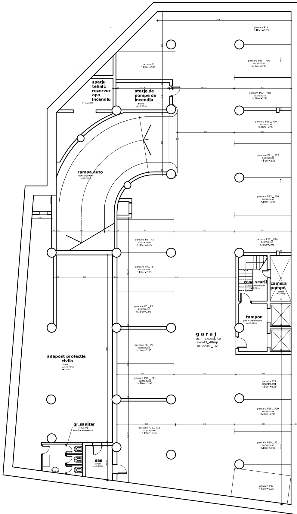
plan subsol S3 _scara 1:200
