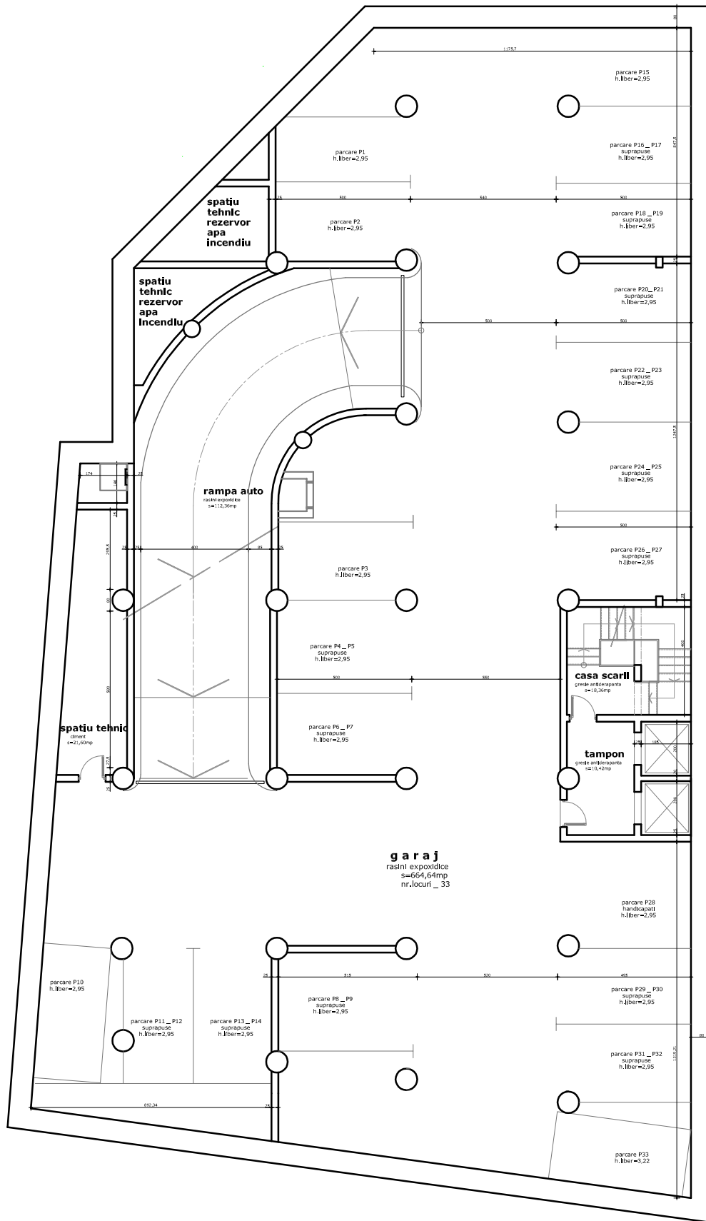
plan subsol S2 _ scara 1:200
